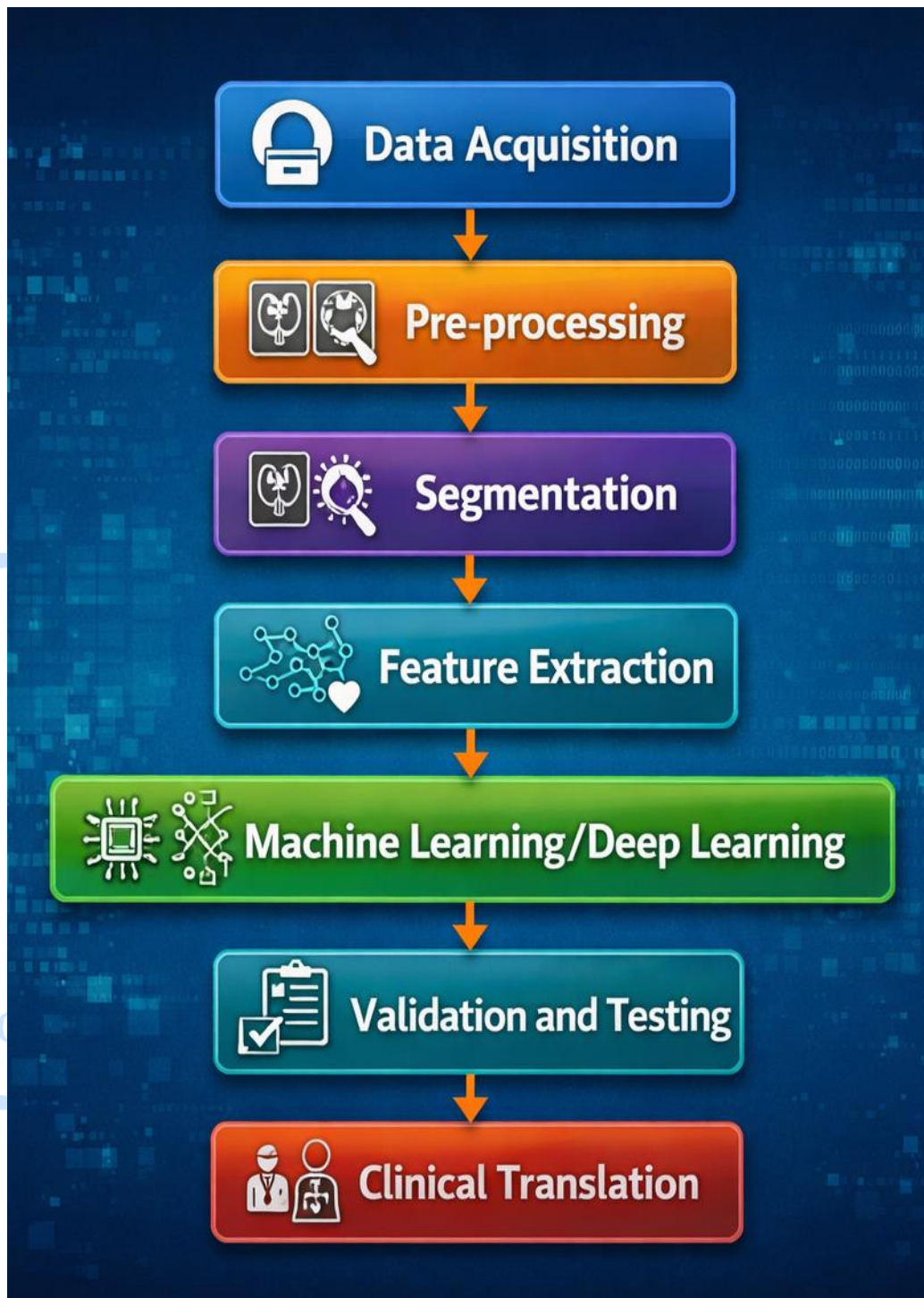
Figure 2: Methodology
