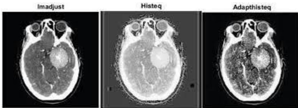
Figure 3: Image Datasets
